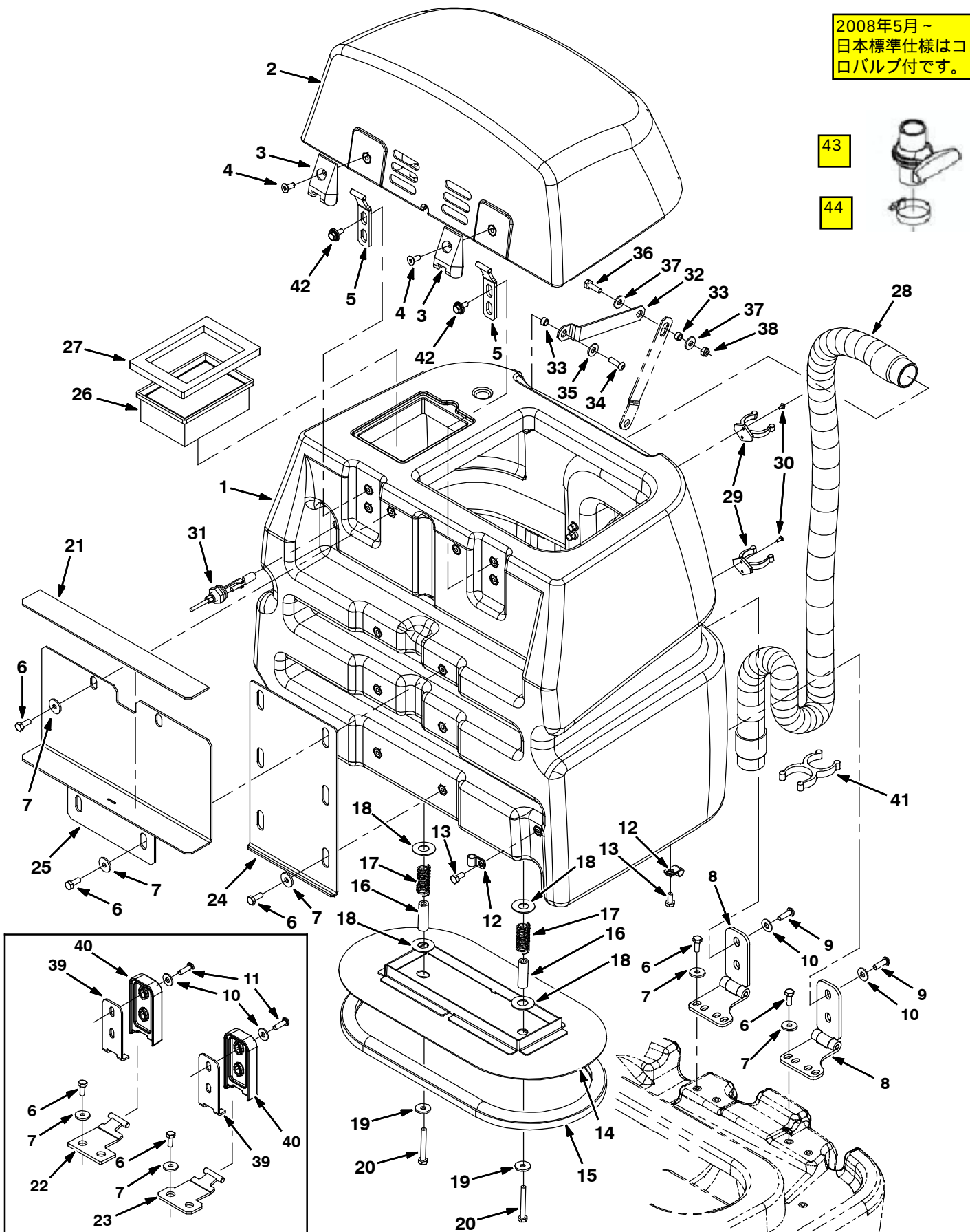
Fig. 26 - Recovery Tank Group
