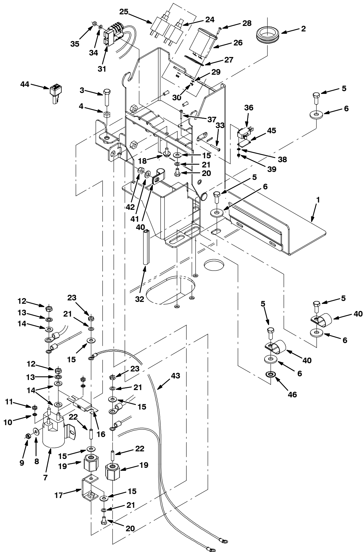
Fig. 38 - Electrical Group
