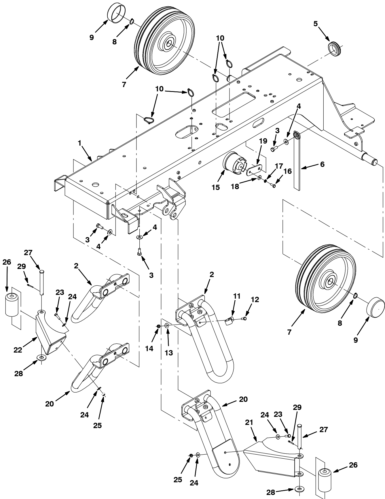
Fig. 6 - Main Frame Group, Cylindrical Scrub Head (S/N 00000000-10448498)
