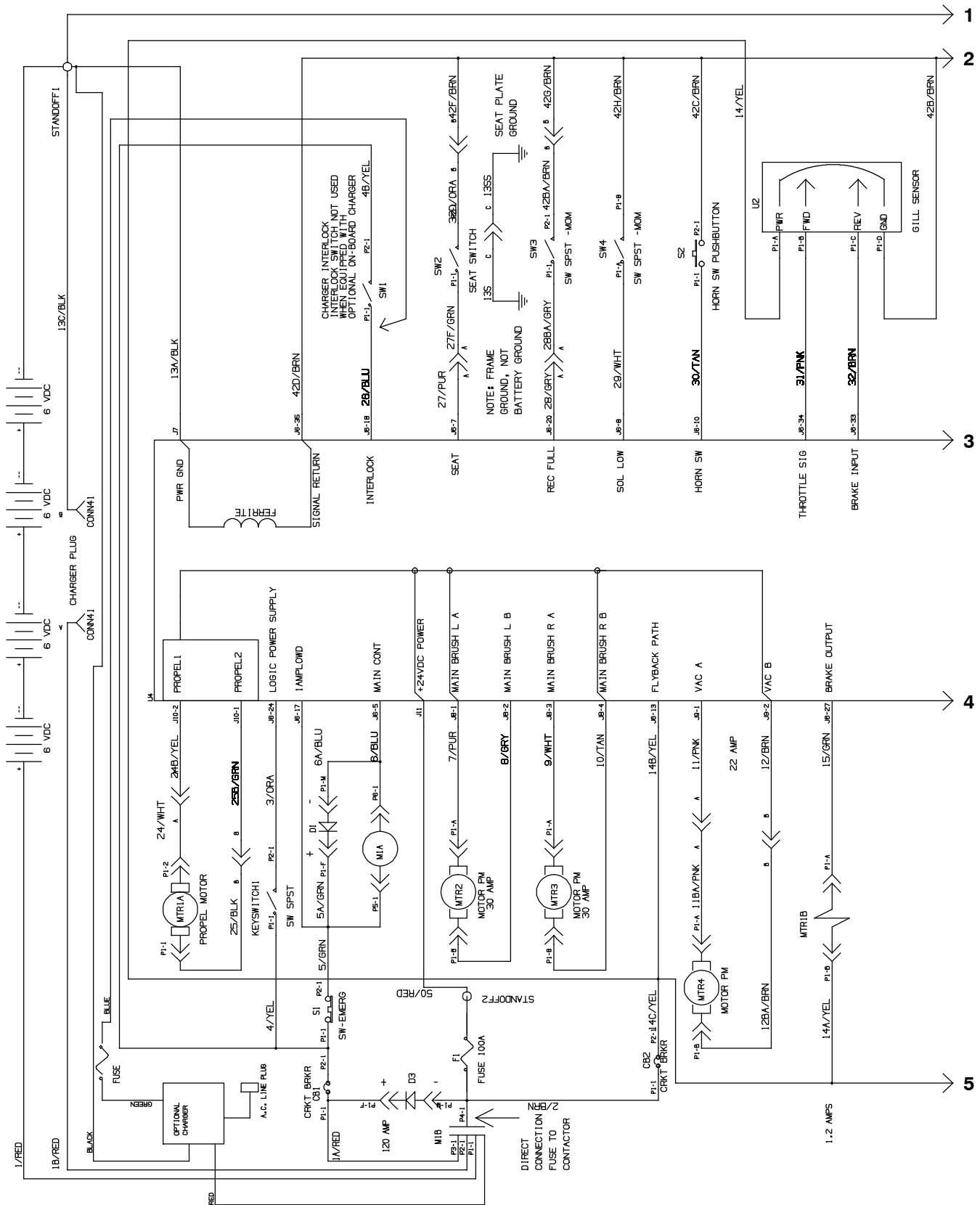
Fig. 40 - Electrical Schematic, Standard &amp; FaST Model (S/N 00000000-10426042)
