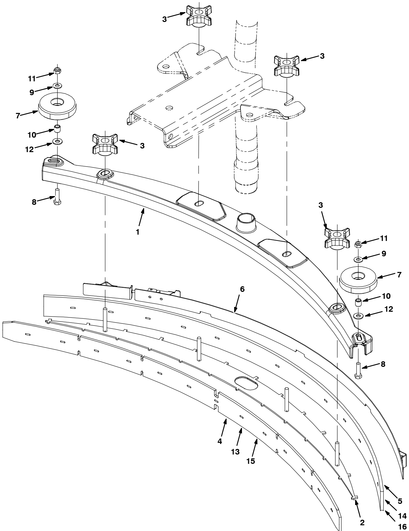
Fig. 36 - Rear Squeegee Group, 800 mm (32 in)
