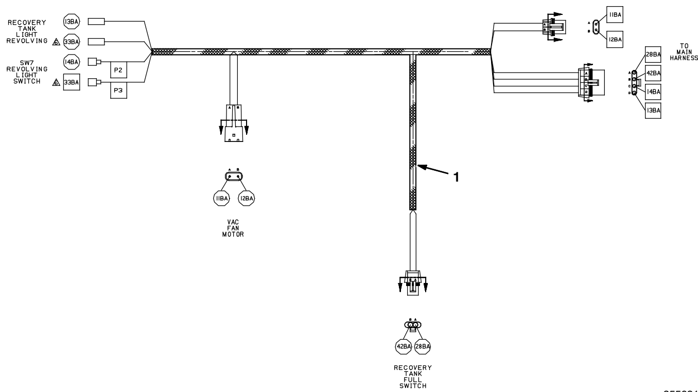
Fig. 45 - Wire Harnesses Group, Tank
